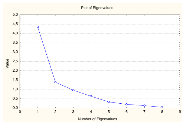
Figure 1. Factor stucture (Eigenvalues)
